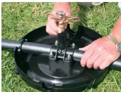
Screw sprinkler into sprinkler riser.
